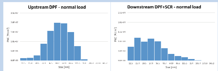
Figures 5 and 6: Average PSD for the asphalt paver, averaged over several measurement cycles of normal operating conditions and measured with NanoScan SMPS. PSD are shown in the full measuring range of 10-420 nm. Note that the scales on the y-axes differ by a factor of 1,000 on the two figures
